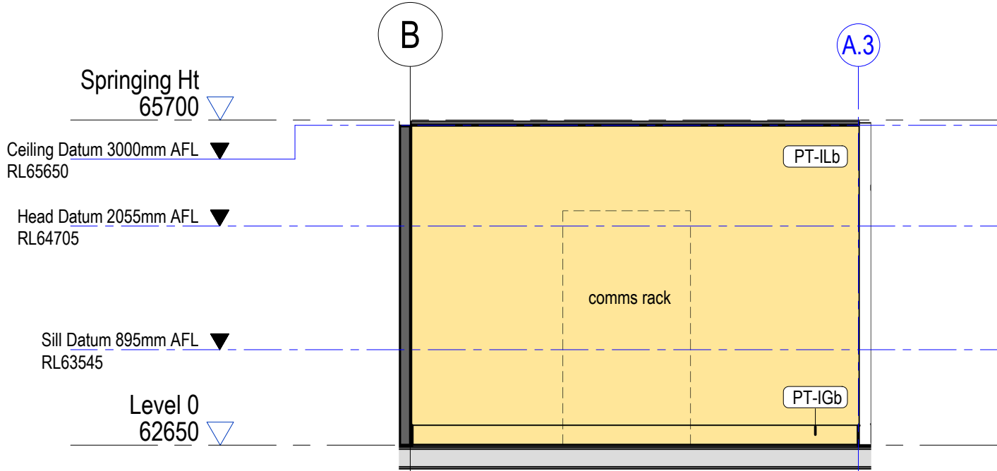
4 0.13 - Comms - South Elevation 1 : 50
