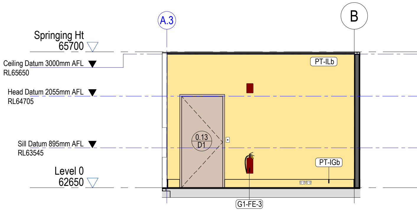
2 0.13 - Comms - North Elevation 1 : 50
