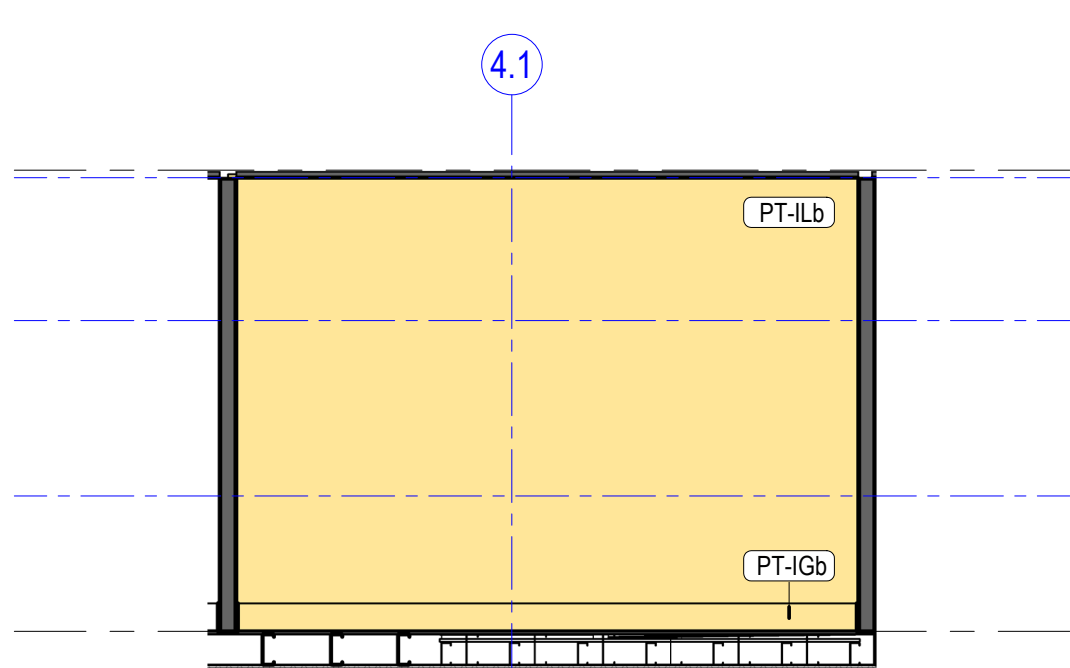
5 0.13 - Comms - West Elevation 1 : 50
