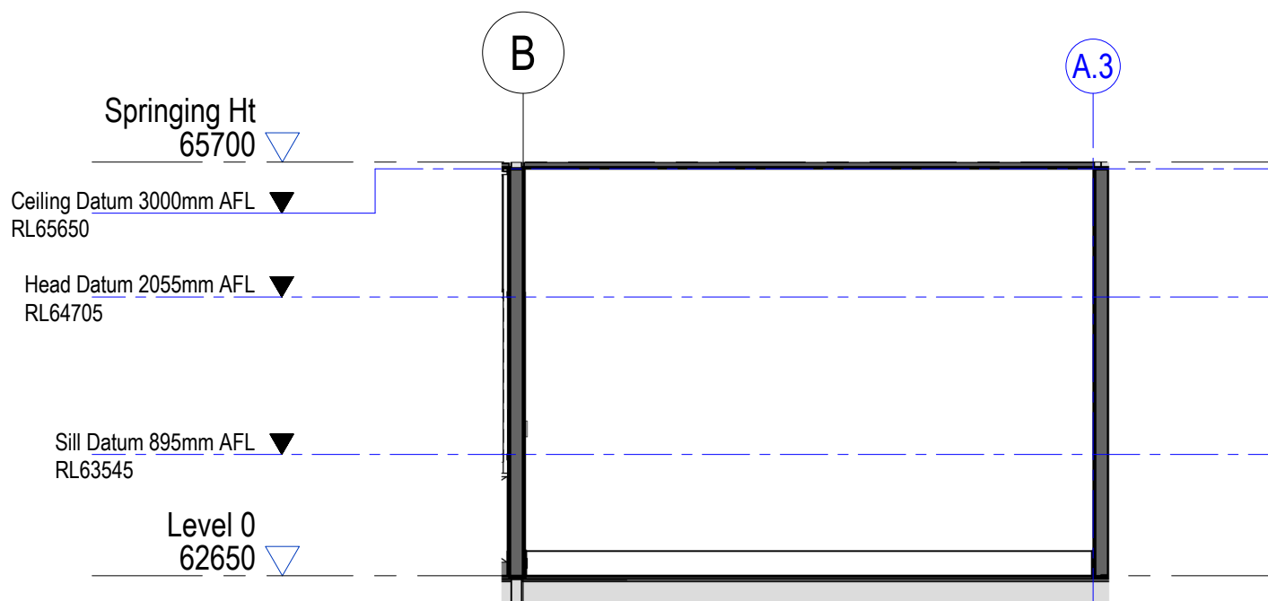
9 0.12 - Store - South Elevation 1 : 50
