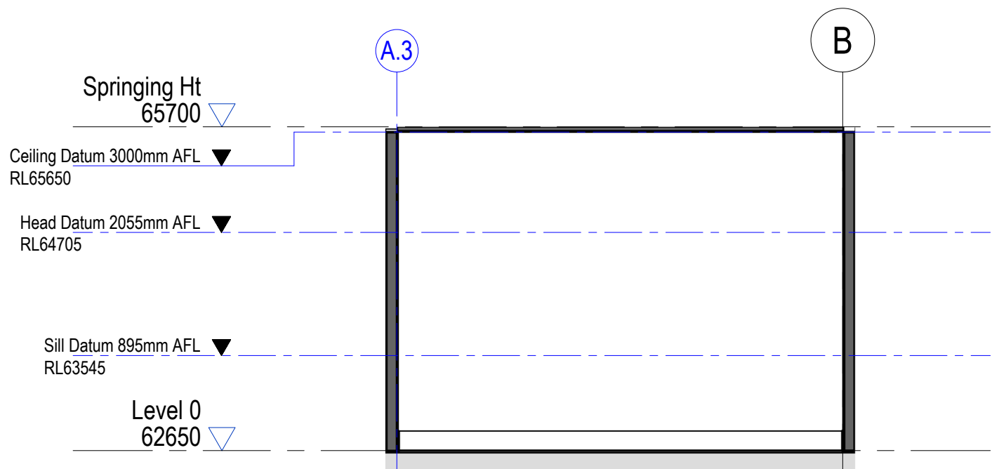
7 0.12 - Store - North Elevation 1 : 50
