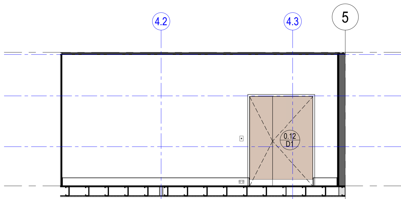
8 0.12 - Store - East Elevation 1 : 50
